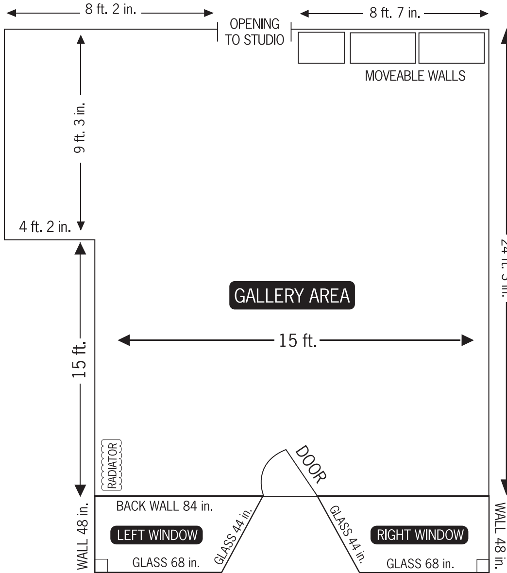
SHOP WINDOWS LAYOUT (VIEW FROM INSIDE GALLERY)
